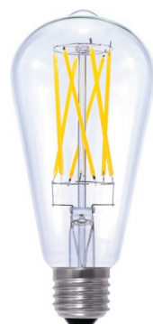
DS700 E27 6,5W 650 lm 2700K Erp F Vetro Chiaro Clear Glass Dimmerabile Dimmable h 145mm Ø 65mm
