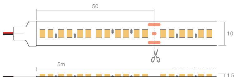
CCT Tunable White 24 W/m 5m bobina in carta paper reel
