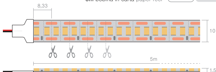
Alta efficienza High efficacy 20 W/m 5m bobina in carta paper reel
