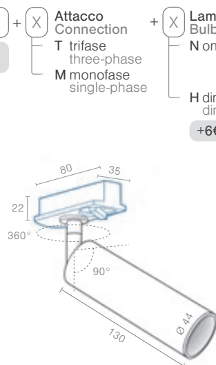
per binario monofase for single-phase track
