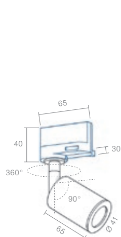
per binario trifase for three-phase track
